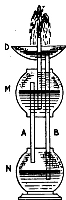
FIG. 2.—Hero's fountain.
